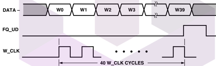
Figure 12. Serial Load Frequency/Phase Update Sequence
